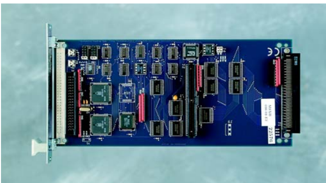
MSXB 036 Counter/Timer
